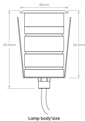
Lamp body's size
