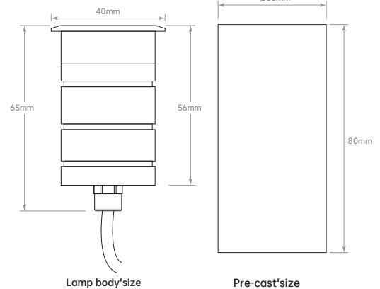
Pre-cast's size
